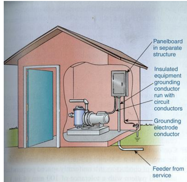
Exhibit 680.9 Grounding requirements per 680.25(B)(2) for remote panelboard and swimming pool equipment located in a structure remote from the service equipment.
